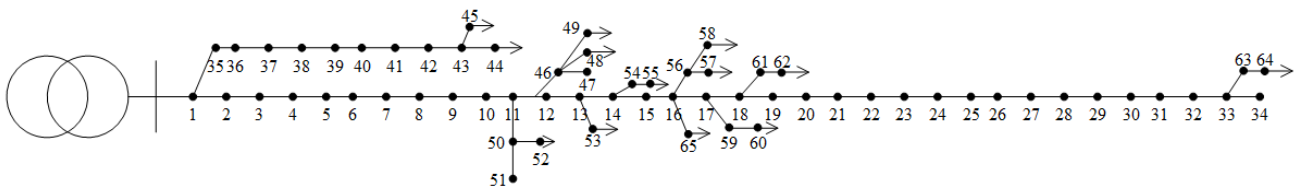
Figure.4. The topology of distribution network
